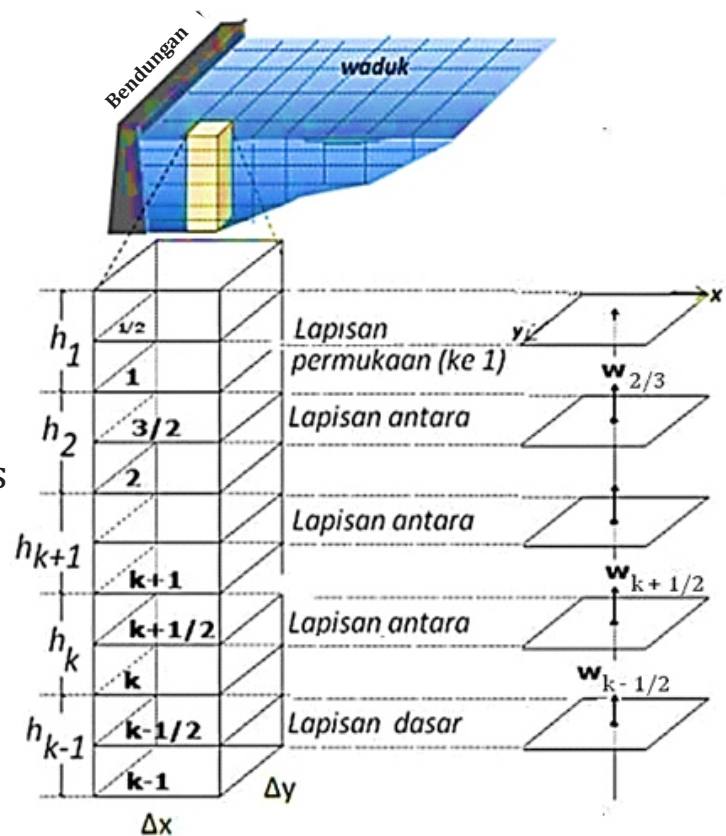
Postur Tegak Badan Air Waduk Model 2-dimensi Berlapis
